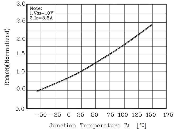
T_j - R_{DS(on)}(\text{Normalized}) Characteristics
