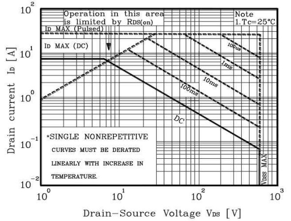
SOA Characteristics
