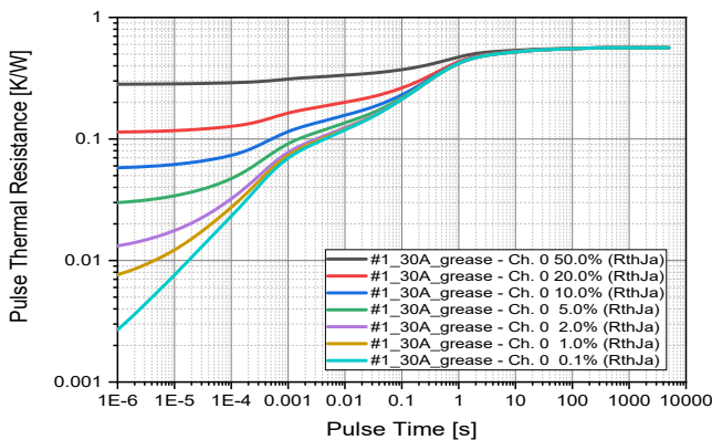
t p – Z th(j-c) Characteristics
