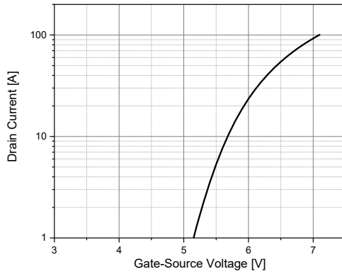
V GS – I D Characteristics, T j =25°C
