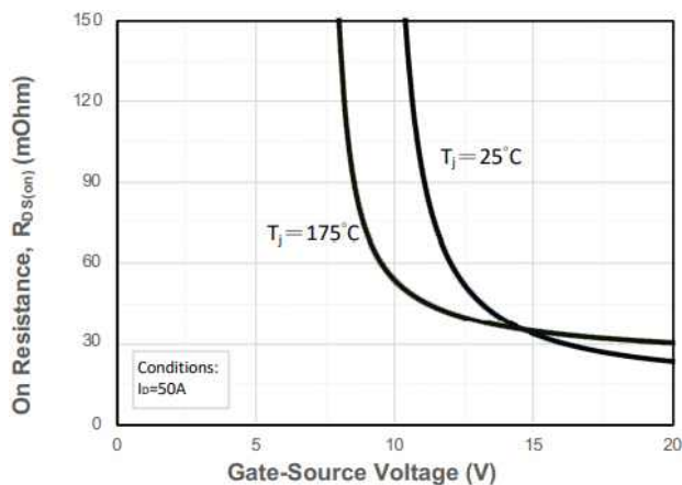
V_{GS} - R_{DS(on)} Characteristics
