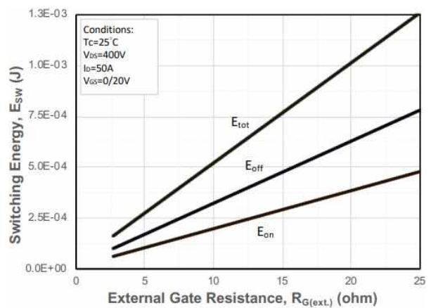
R G(ext) – E SW Characteristics
