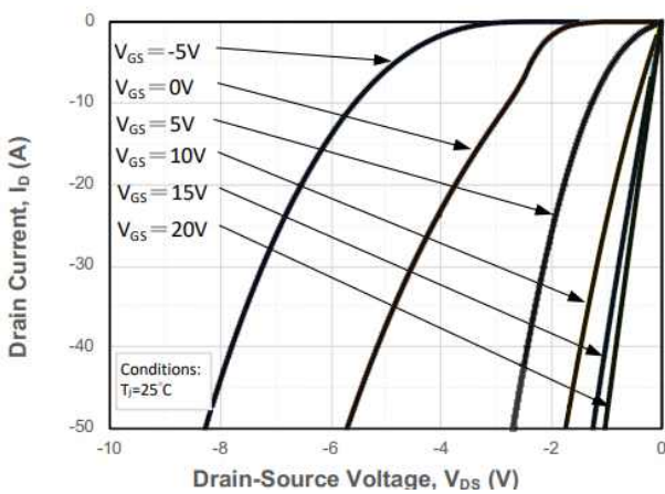
V_{DS} - I_D Characteristics, T_j = 25^\circ\text{C}
