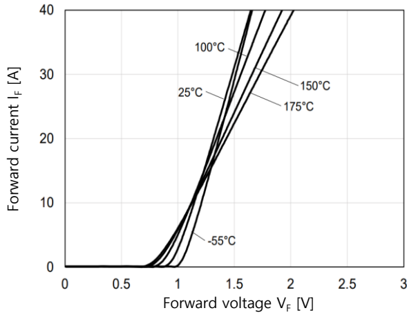
V_F - I_F Characteristics
