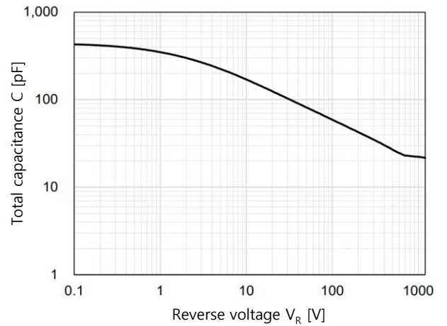
V_R - C Characteristics
