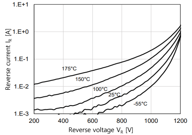
V_R - I_R Characteristics
